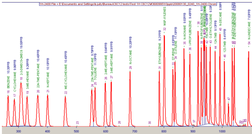
An example chromatogram (C6-C12)
